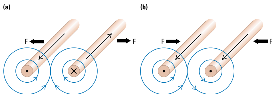
Figure 4 (a) If the electric currents in the parallel wires are in opposite directions, the force is repulsive. (b) If the electric currents in the parallel wires are in the same direction, the force is attractive.
