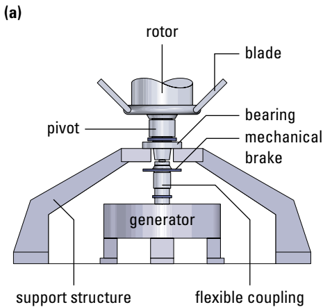
Figure 7 Wind energy
