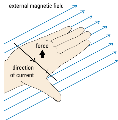
Figure 2 The right-hand rule for the motor principle
