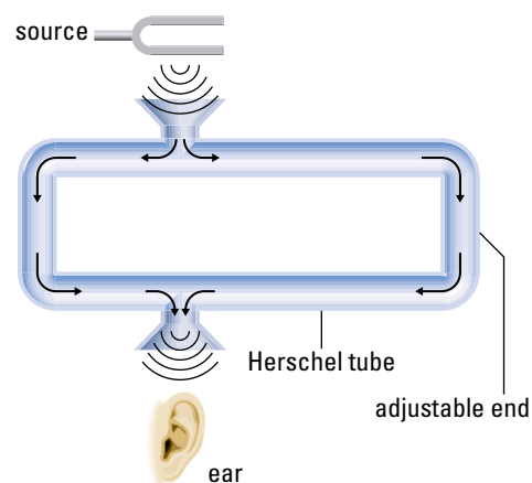
Figure 4 A Herschel tube
