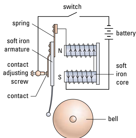
Figure 10 An electric bell
